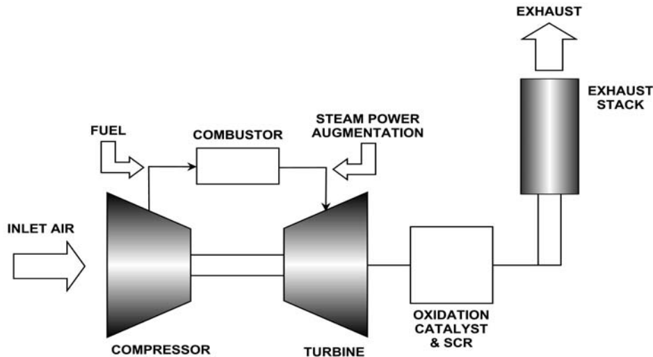
CTG Process Flow Diagram
